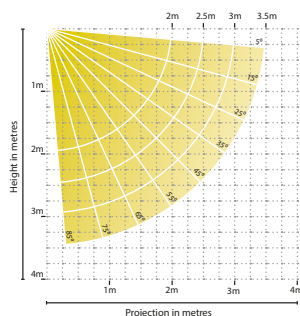
ARM PROJECTION
